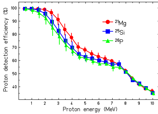
Fig. 4. GEANT simulation of the proton detection efficiency of the implantation detector E4 . The error bars on the plotted data are deduced from different parametrizations of the ion implantation profiles. An uncertainty due to the detector thickness is not included, as it is of the same order of magnitude as the uncertainty of the implantation profile (see text for details).
