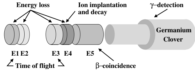
Fig. 2. Schematic view of the identification and detection set-up. It includes a germanium detector and five silicon detectors mounted in close geometry, where selected ions were identified by means of energy loss and time-of-flight measurements. The last two detectors were used to observe the charged particles emitted in decay events in the implantation detector E4 .
