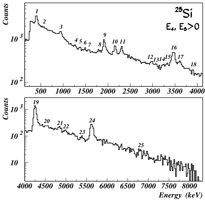
Fig. 6. \beta -delayed proton spectrum obtained in coincidence with a signal in E5 in the decay of ^{25}\text{Si} . The peak labels correspond to the peak numbers used in tables 2 and 3.
