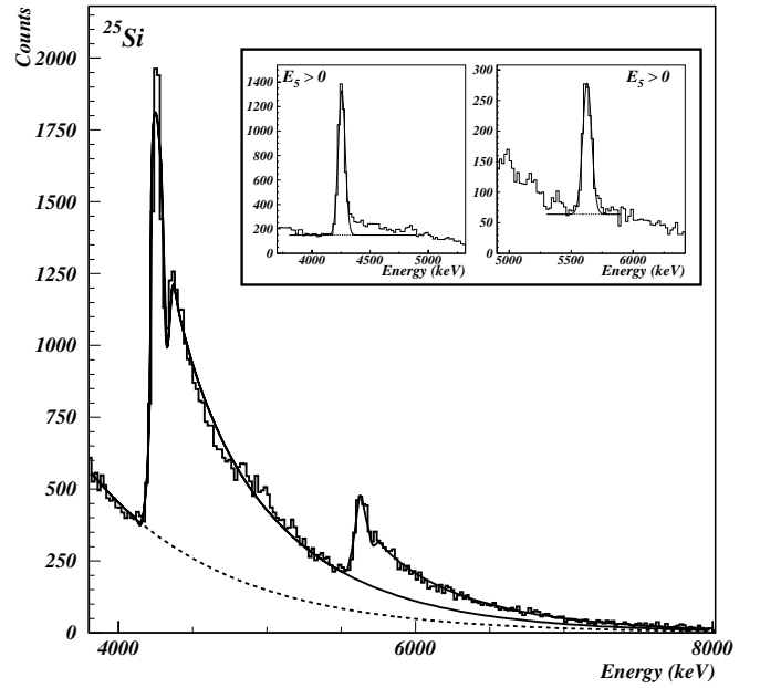
Fig. 5. High-energy part of the \beta -delayed proton spectrum in the decay of ^{25}\text{Si} . The areas of the two main proton peaks above 4 MeV obtained with (inset) and without (main figure) coincidence condition were used to extract an average normalization factor Kc_p for the setting on ^{25}\text{Si} .
