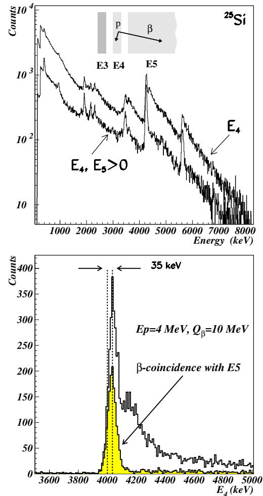
Fig. 3. The upper part of the figure shows the influence of the \beta coincidence condition ( E5 > 0 ) on the energy spectrum delivered by the detector E4 for the setting on ^{25}\text{Si} . The lower part of the figure presents a GEANT simulation of the effect of the coincidence condition on the shape of a \beta -delayed proton emission peak. The dotted lines show the 35 keV energy shift due to the \beta pile-up, i.e. a 4 MeV proton peak is in fact observed at an energy of 4.035 MeV. This shift depends on the implantation depth and varies for the different nuclei studied in this work. The coincidence condition does not alter this shift significantly.
