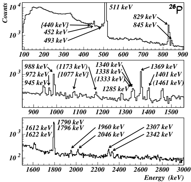
Fig. 11. \gamma -decay spectrum of ^{26}\text{P} : background \gamma lines from ^{60}\text{Co} and ^{40}\text{K} are indicated within round parentheses. \gamma -rays within curly brackets are due to the contaminating nuclei ^{23}\text{Mg} and ^{24}\text{Al} . All other \gamma lines are related to the \beta -decay of ^{26}\text{P} , except the one at 1285 keV which could not be attributed.
