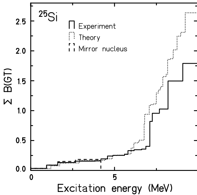
Fig. 9. Theoretical and experimental distributions of the summed Gamow-Teller strength ( \Sigma B(\text{GT}) ) for the decay of ^{25}\text{Si} . At low excitation energy, the distributions are also compared to the one obtained from the mirror \beta -decay of ^{25}\text{Na} assuming isospin symmetry. The error of the Gamow-Teller strength distribution as determined in the present work is about 20%.
